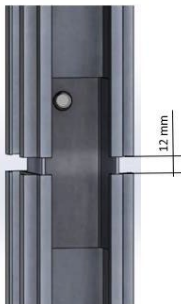
Figure 4d- Raccord dilatant entre deux rails verticaux ISOPLI NG 36
