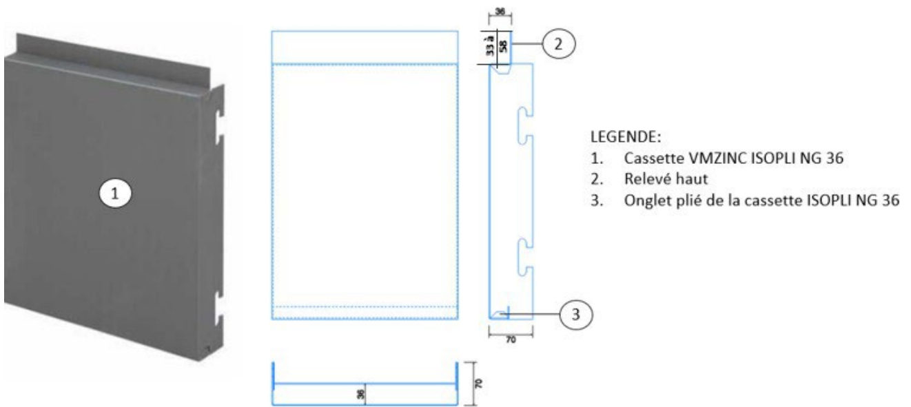
Figure 1d - Cassette ISOPLI NG 36 verticale
