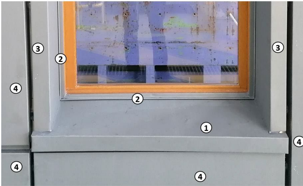
Figure 24 e – Appui de baie
