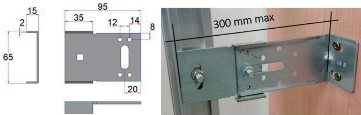
Figure 2d – Rallonge ISOLCO point coulissant
