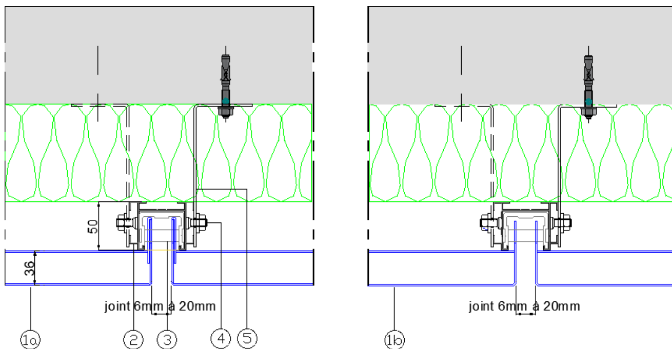
Figure 2d – Rallonge ISOLCO point coulissant
